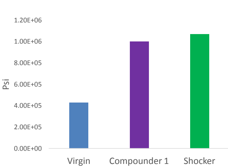
Flexural Modulus (Psi)
