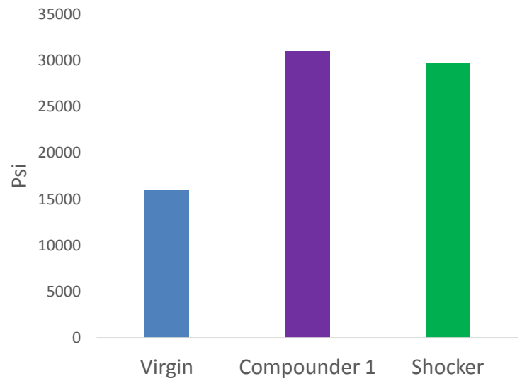
Flexural Strength (Psi)
