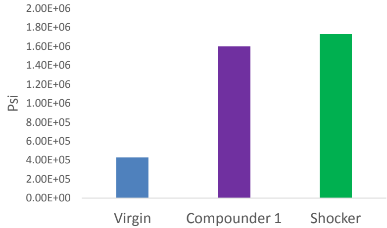
Flexural Modulus for 20% CF and PA (Psi)
