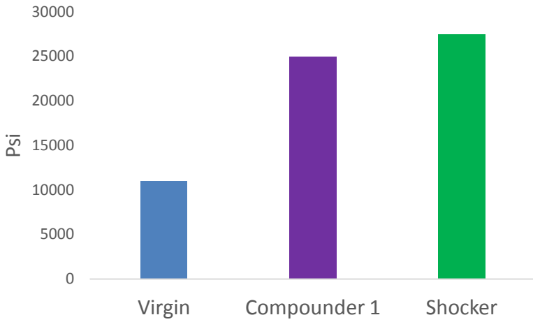
Tensile Strength for 20 % CF and PA (Psi)
