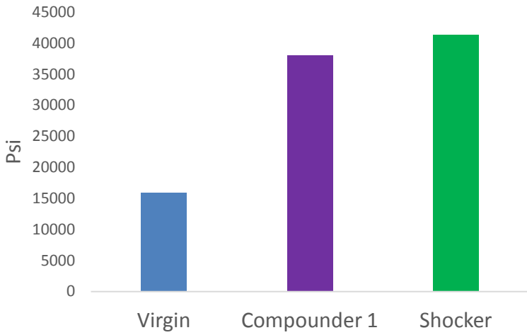
Flexural Strength for 20% CF and PA (Psi)
