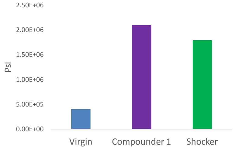
Tensile Modulus for 20% CF and PA (Psi)
